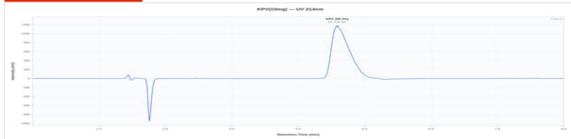
KPV 10mg - FRP-578100626: UV Chromatogram
